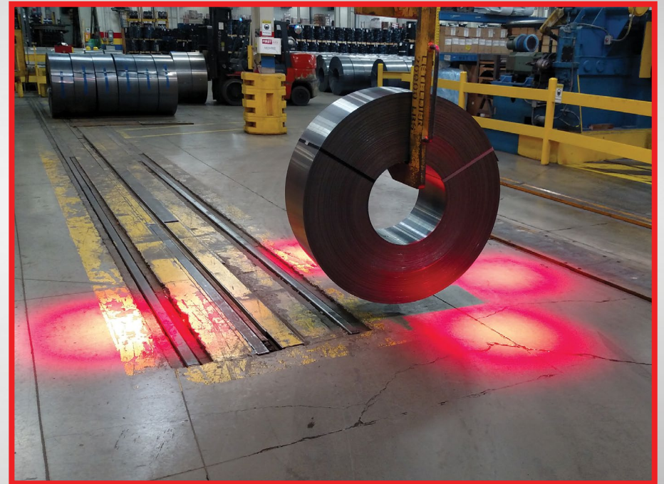
Four spot configuration (available in red or blue or a mix)
